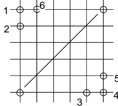
Pin arrangement (View in mounting direction)
