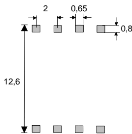
Terminal dimensions at soldering point.
