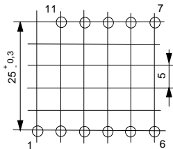
Pin arrangement (View in mounting direction)
