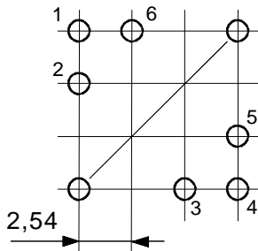
Pin arrangement (View in mounting direction)
