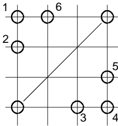
Pin arrangement (View in mounting direction)
