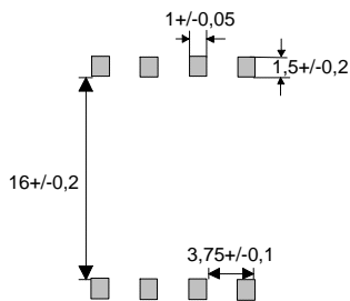
Terminal dimensions at soldering point.
