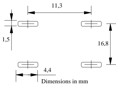
Pin arrangement (View in mounting direction)
