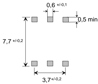
Terminal dimensions at soldering point.
