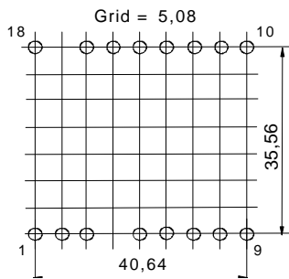
Pin arrangement (View in mounting direction)
