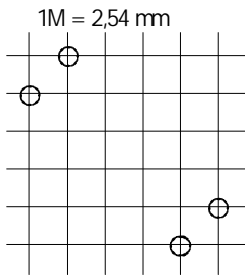
Pin arrangement (View in mounting direction)
